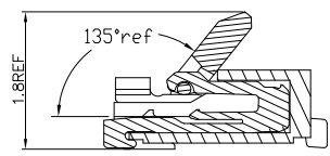
When Actuator Is Opened Scale 2:1
