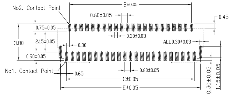
FPC/FFC Insert Direction Recommended P.C.B Layout
